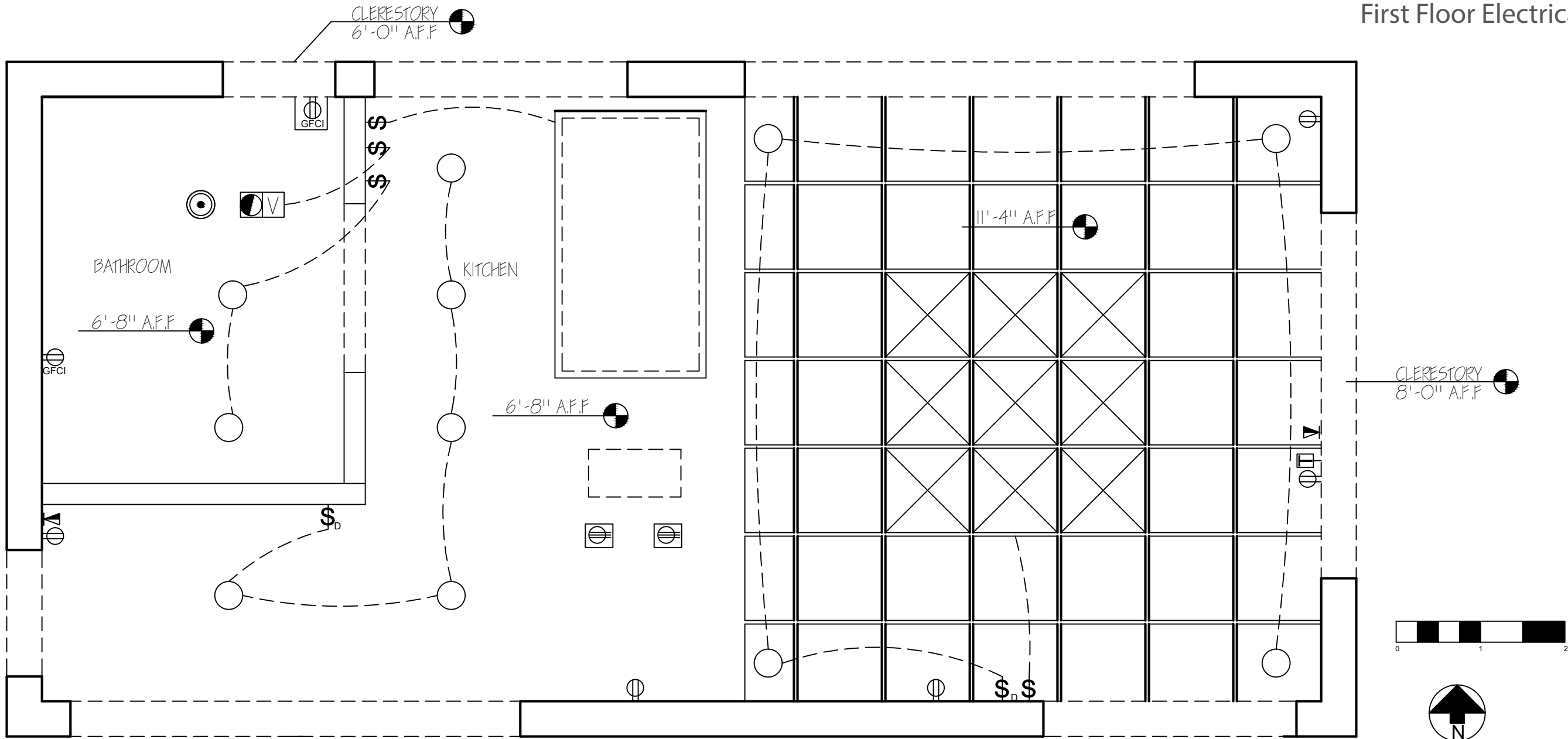
FIRST FLOOR ELECTRICAL PLAN
