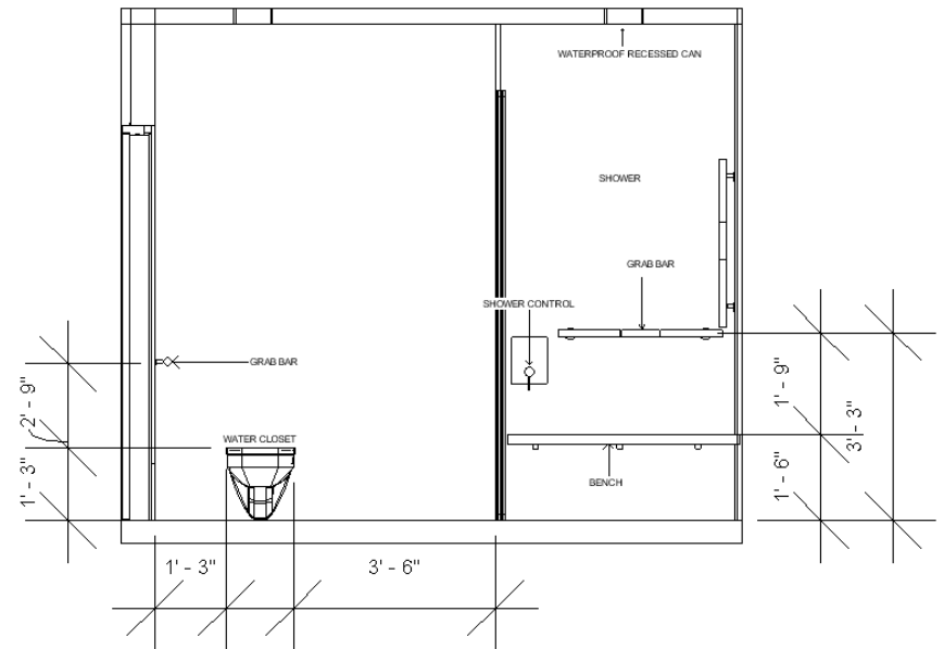
WATER CLOSET ELEVATION
