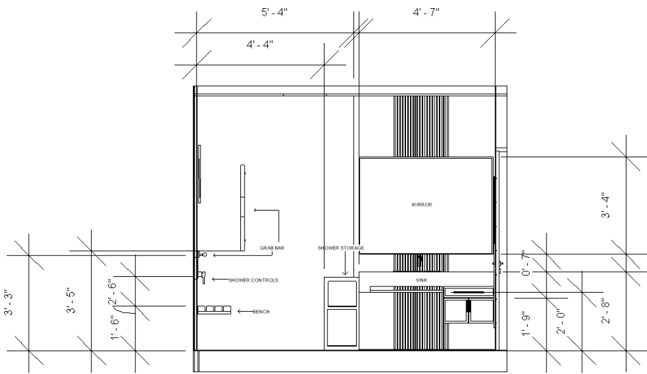
SHOWER ELEVATION
