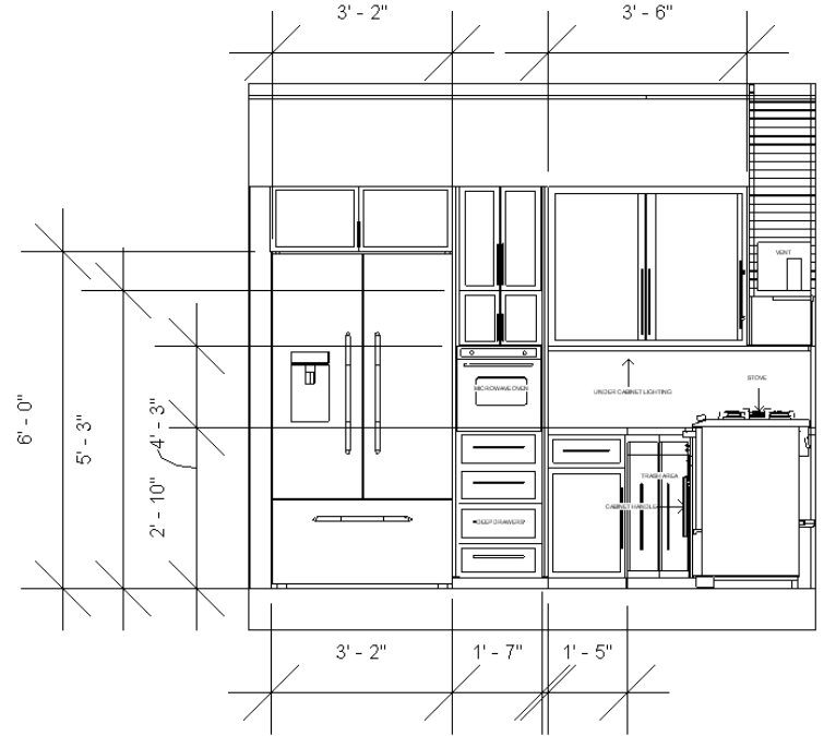
KITCHEN ELEVATIONS
