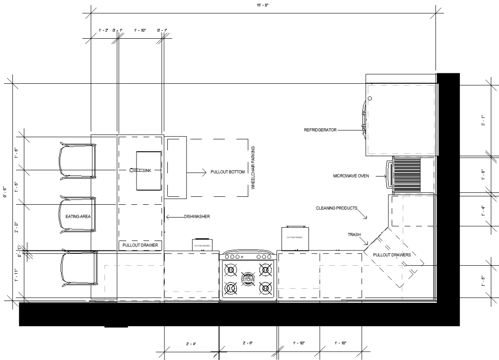
ENLARGED KITCHEN PLAN
